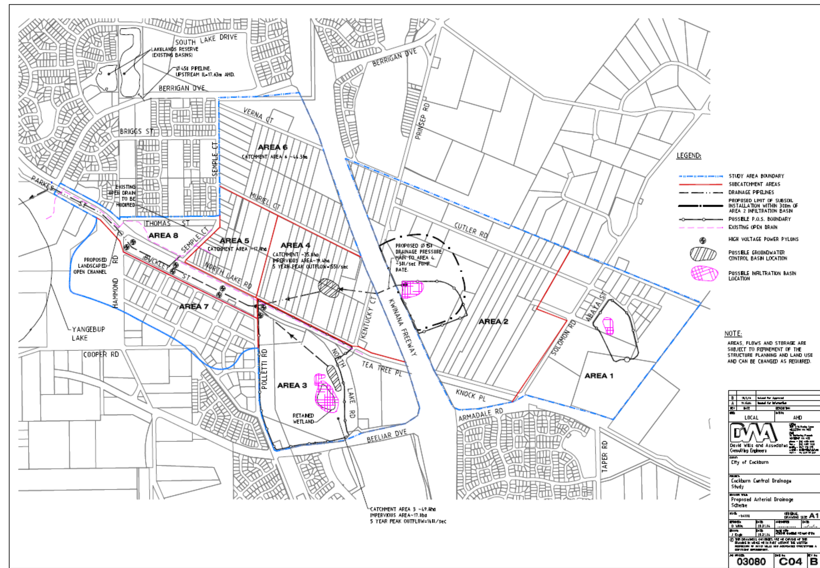
Map Solomon Arterial Drainage Scheme
