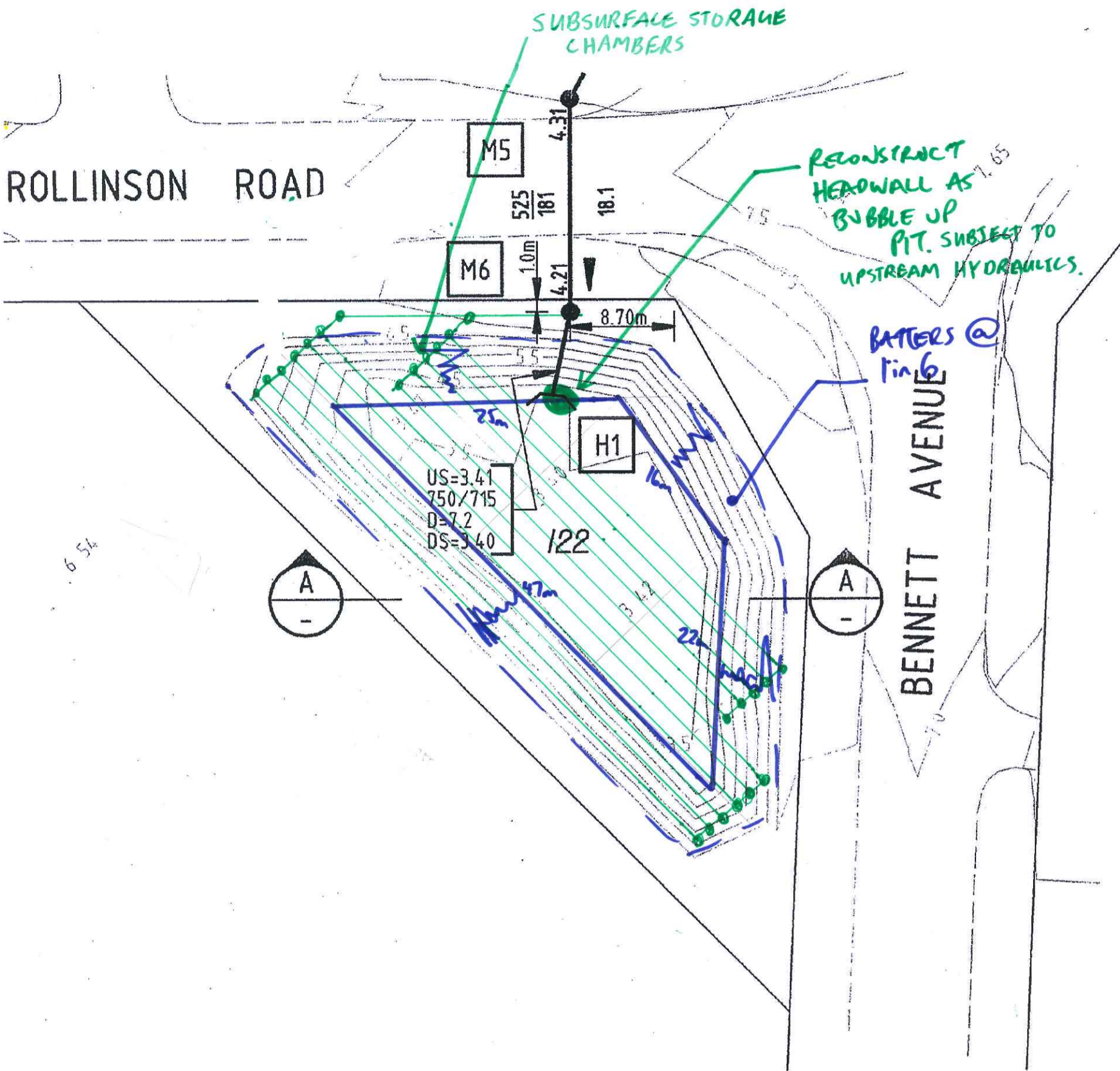
PLAN SCALE 1:500
