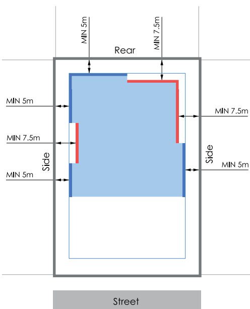
Figure 7.2.1.1: Tower setbacks to side and rear boundaries illustration
