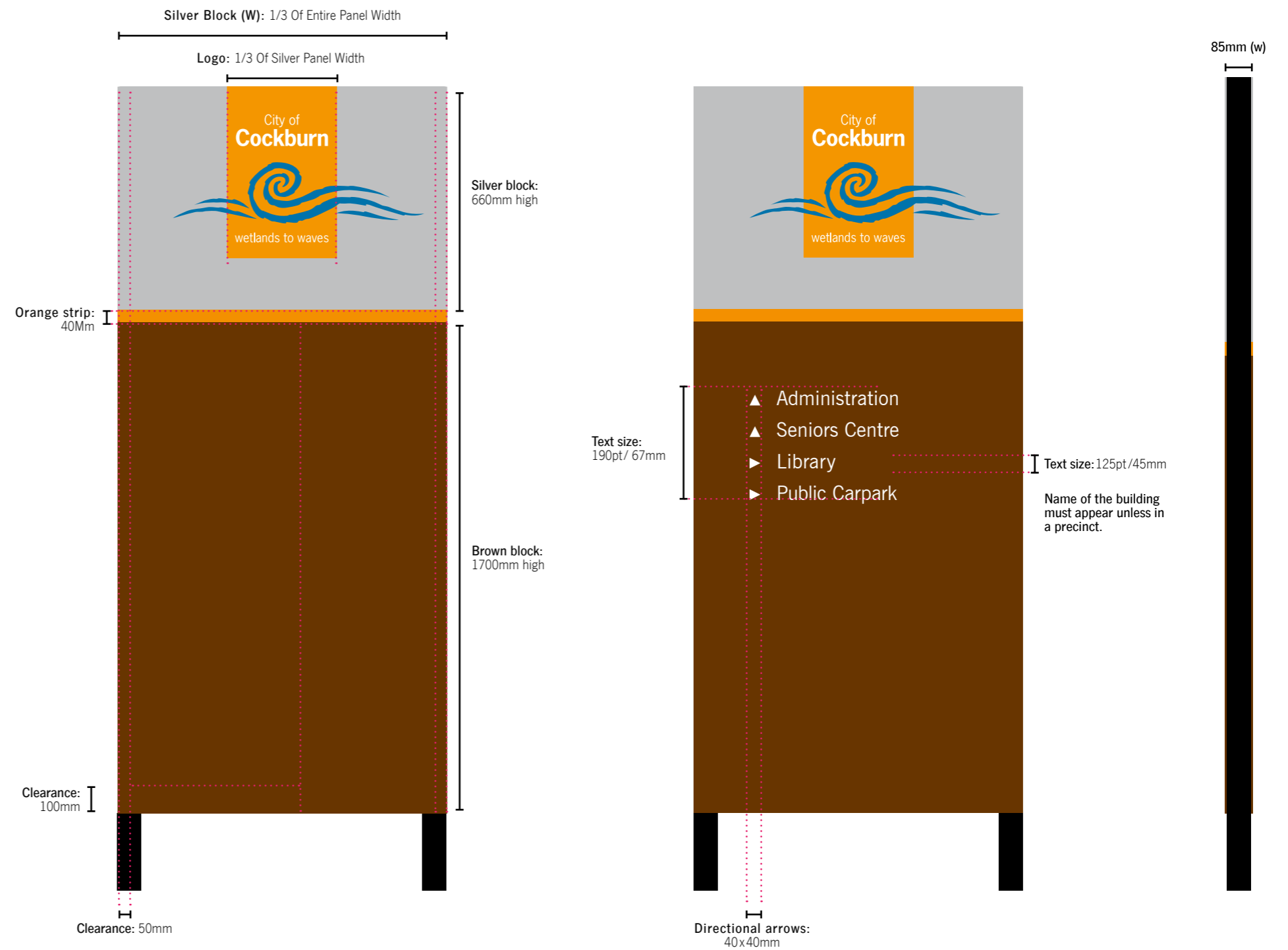
Side view
