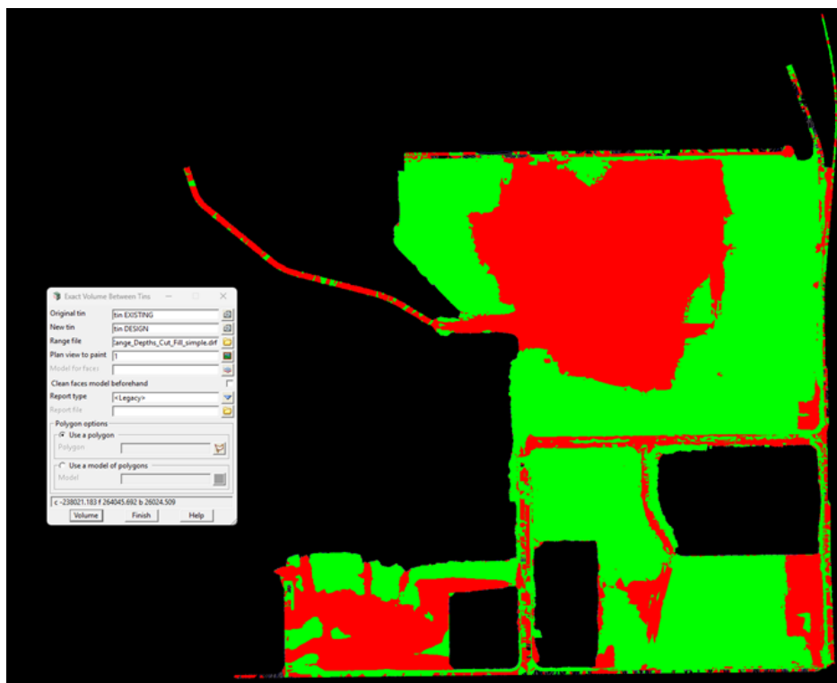
Figure 11 Indicative Cut areas (red) and fill areas (green)
