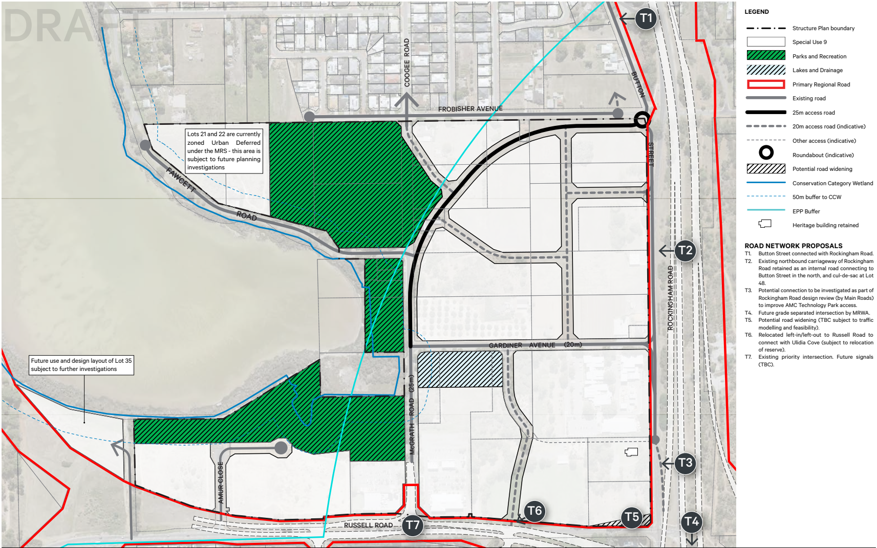
Structure Plan (Ultimate – after Rockingham Road Expressway/FRAH is constructed) Australian Marine Complex - Technology Precinct
