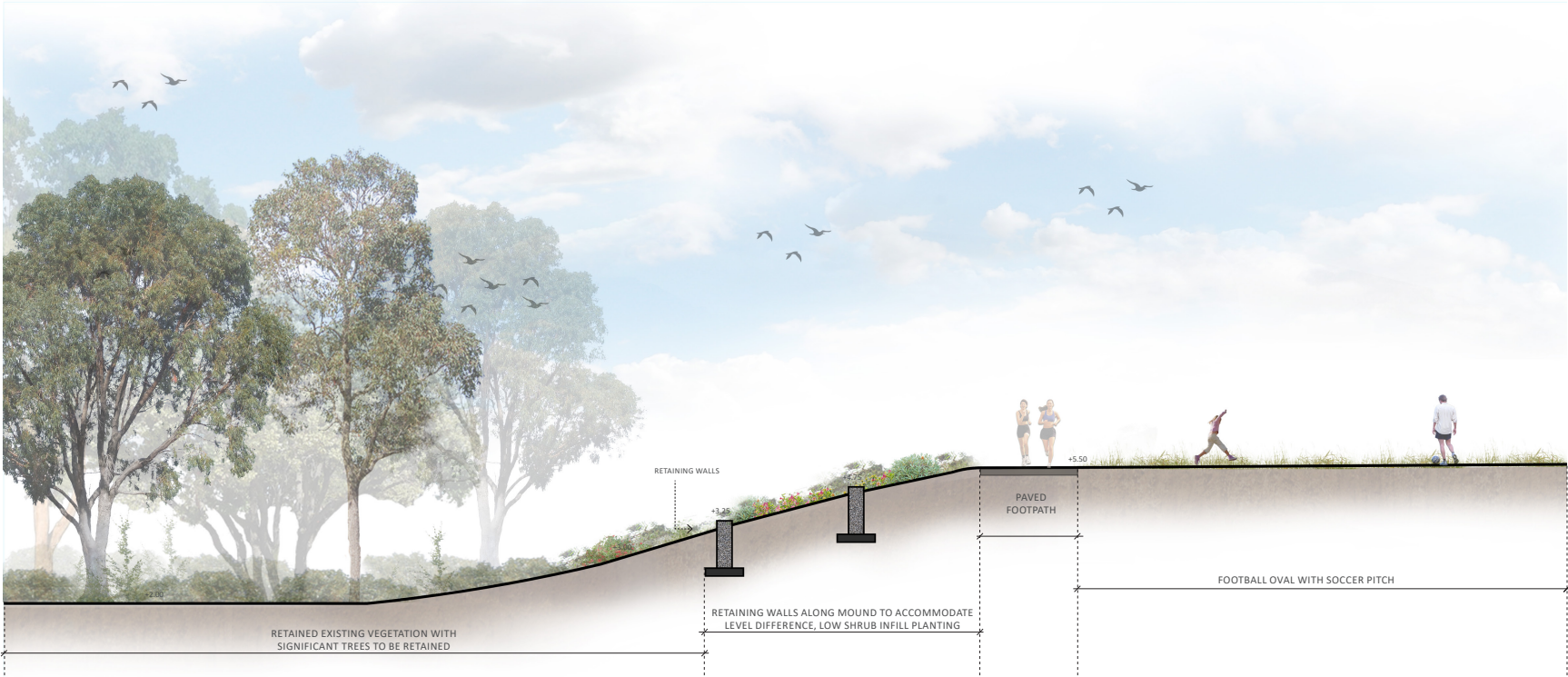
SECTION B-B
