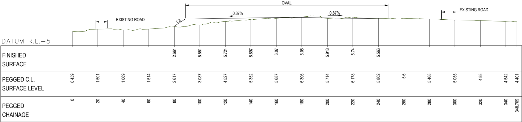
OVAL SECTION 1:1000 HOR, 1:500 VER
