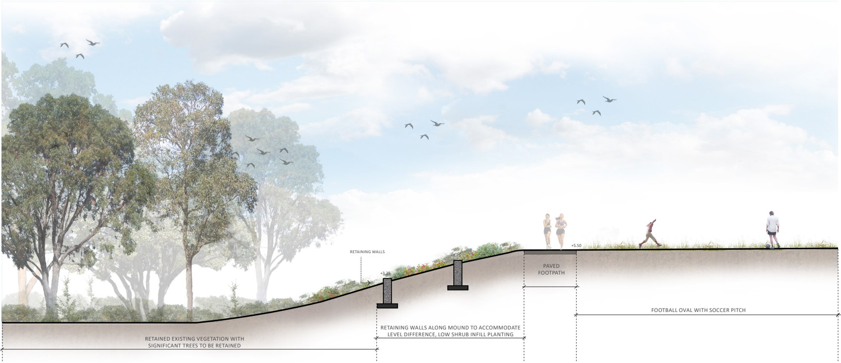
SECTION B-B
