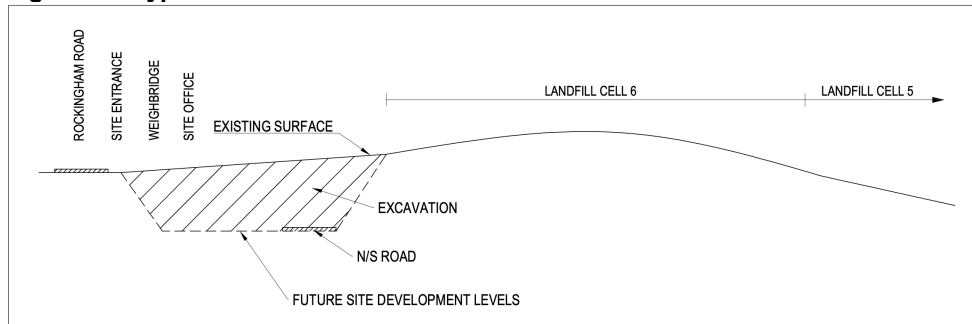
Figure 1 – Typical Cross-Section
